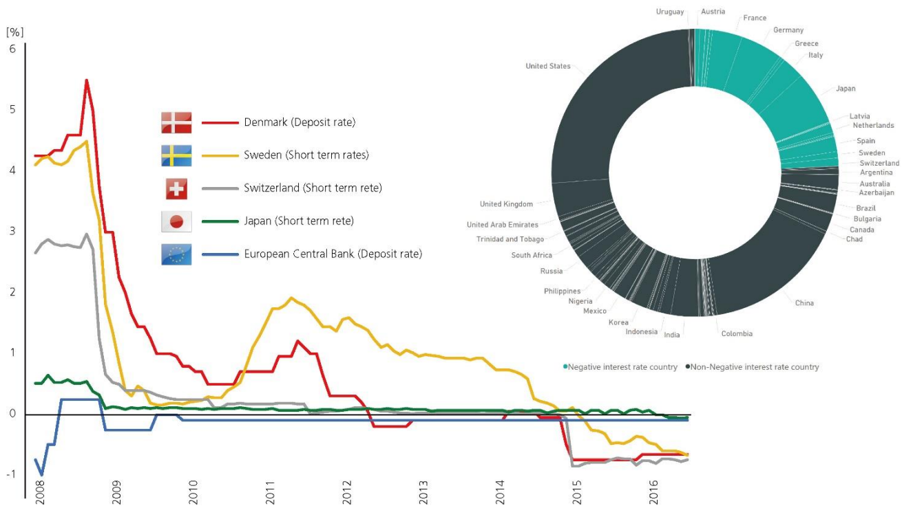
Figure 1: Era of negative interest rates: Interest rate time series of major countries/region during 2008-2016 (Left) Proportion of global GDP governed by a central bank with negative interest rates (Right)
